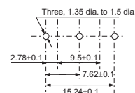
PCB Mounting Dimensions (Reference)
